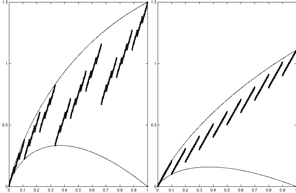
FIGURE 3. Graphs of y = H_B(x) , y = x \log_B(1/x) , and y = Bx/(B-1) + x \log_B(1/x) on [0, 1] for the values B = 3 and B = 10 .
